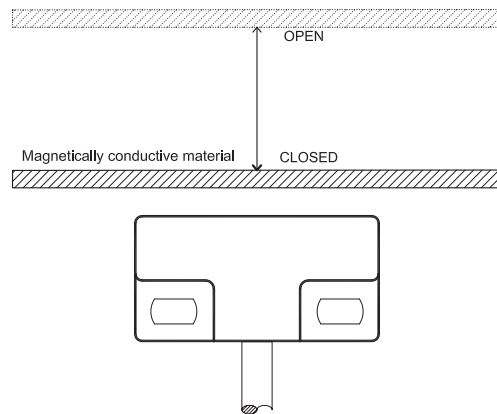
Fig. #36 Standex Electronics has designed a patented bridge sensor requiring no external magnets. When the sensor is brought close to a ferromagnetic sheet or plate the sensor contacts will close. When the sheet is withdrawn, the contacts will open.
