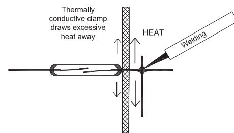
Fig. #4 Use of Heat Sinking or preheating Reed Switches for soldering or welding can prevent heat stress damage.
