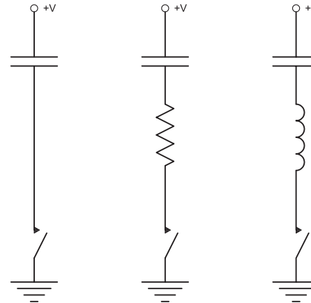
Fig. #7 Switching capacitance directly will damage the contacts rapidly with high inrush currents. Adding a resistor or an inductor will reduce the inrush current and reduce the contact wear.
