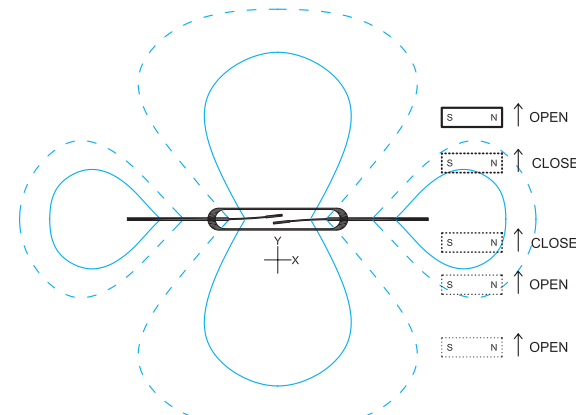
Fig. #28 The closing, holding, and opening are presented for a magnet parallel to the Reed Switch, but moving perpendicular to the plane of the Reed Switch and being influenced by the outer magnetic lobe.
