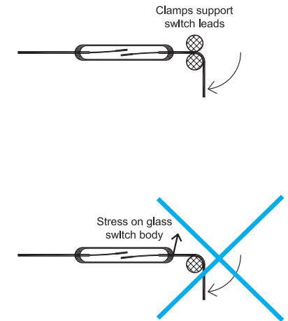
Fig. #1 Presentation of the proper and improper way of bending a Reed Switch. Supporting the switch lead while bending is a must.
