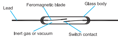
Fig. #1 The basic hermetically sealed Form 1A (normally open) Reed Switch and its component makeup.
