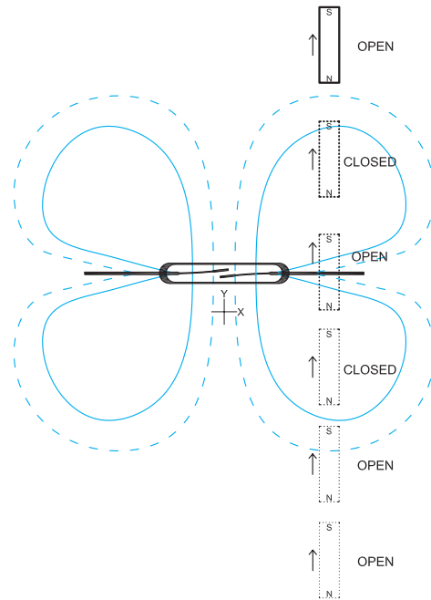
Figure #32 The opening and closing points are shown for a vertically mounted magnet making an approach perpendicular to the axis of the Reed Switch through its end point. Here the Reed Switch will close and open two times.
