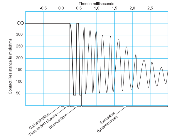
Fig. #12 A dynamic contact resistance pattern portraying excessive dynamic noise indicating potential stressed or cracked glass seal.
