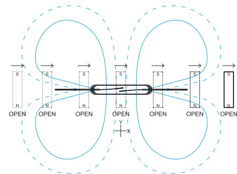
Fig. #31 The opening and closing points are shown for a vertically mounted magnet making an approach parallel to the axis of the Reed Switch. Here the Reed Switch will close and open two times.
