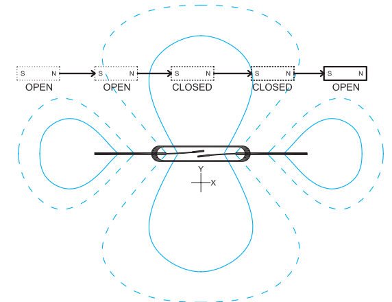
Fig. #24 The opening, closing and holding points are shown for a magnet passing in parallel to Reed Switch and being affected by the center magnetic lobe.
