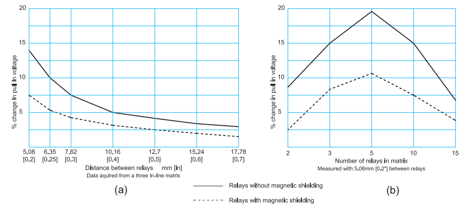
Fig. #6 (a) Percent Pull-In Voltage Increase vs. On-Center Distance Between SIL Relays. Data was taken using the three-relay test matrix (see Figure 5). (b) Percent Pull-In Voltage Increase vs. the Number of Relays in the test configuration, using matrix for up to 15 relays.
