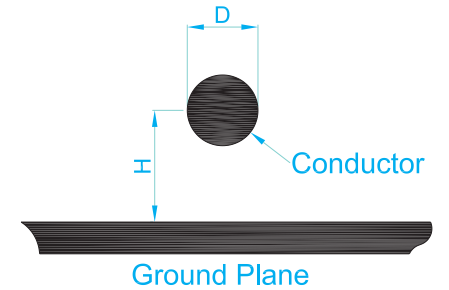
Fig. #11 Round wire over a ground geometry.
