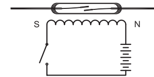
Fig. #1 A Reed Relay consists of a copper insulated wire wound coil with a Reed Switch traditionally mounted on its center axis.
