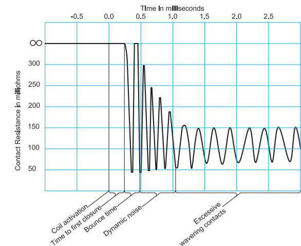
Fig. #13 A dynamic contact resistance pattern with indicated excessive contact wavering often indicates a stressed or cracked glass seal.
