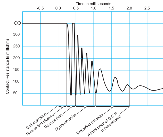
Fig. #10 A typical dynamic contact resistance portrayal showing the first closure, bouncing, dynamic noise and pattern generated by waver-ing contacts
