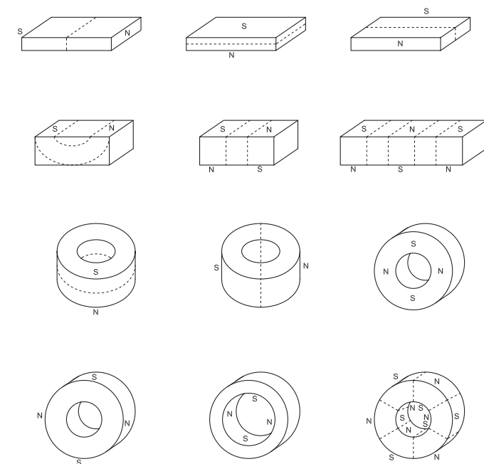
Fig. #1 An assortment of magnets are shown. Magnets can be formed and made into almost any shape.
