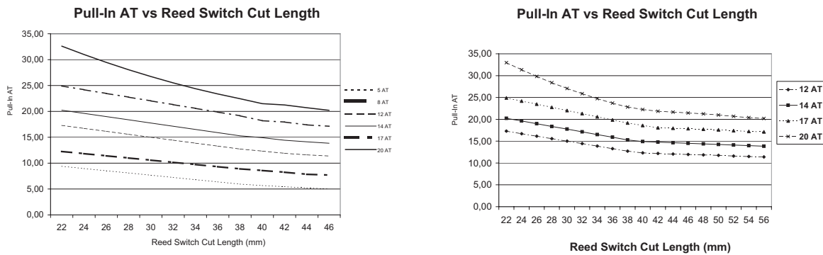
Fig. #2 Presentation of the operate AT change for various cut lengths for a given operate AT.
