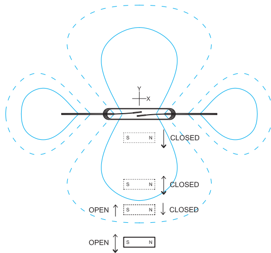
Fig. #27 The closing, holding, and opening are portrayed for a magnet parallel to the Reed Switch, but moving perpendicular to the plane of the Reed Switch and being influenced by the center magnet lobe.
