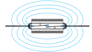
Fig. #4 A Reed Switch sitting in a solenoid where the magnetic field is strongest in its center. Here the reed blades become polarized and an attractive force exists across the contacts.
