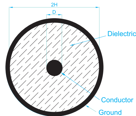
Fig. #10 Coaxial cable geometry
