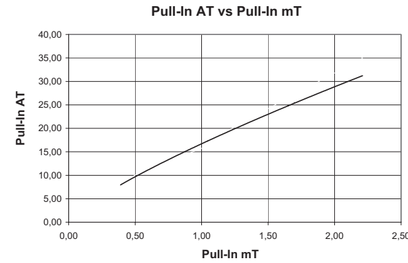
Fig. #5 The Pull-In AT is presented with its corresponding mT Pull-In level.
