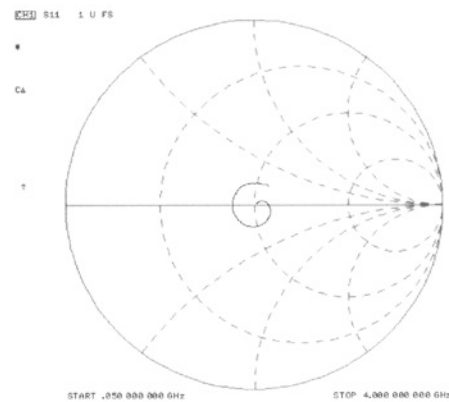
Fig. #25 Shows a Smith Chart plotted for frequencies to 4 GHz. The second dotted circle starting from the right is the 50 Ohm impedance point.
