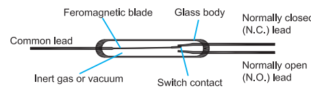
Fig. #2 The 1 Form C (single pole double throw) three leaded Reed Switch and its component makeup.
