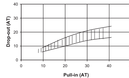
Fig. #7 The Pull-in and Drop-out ranges are shown. Note that variation in hysteresis is for low ampere turns (AT) is very small and increases with higher AT.
