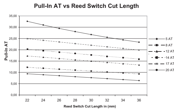
Fig. #4 Presentation of the operate AT change for various cut lengths for a given operate AT.
