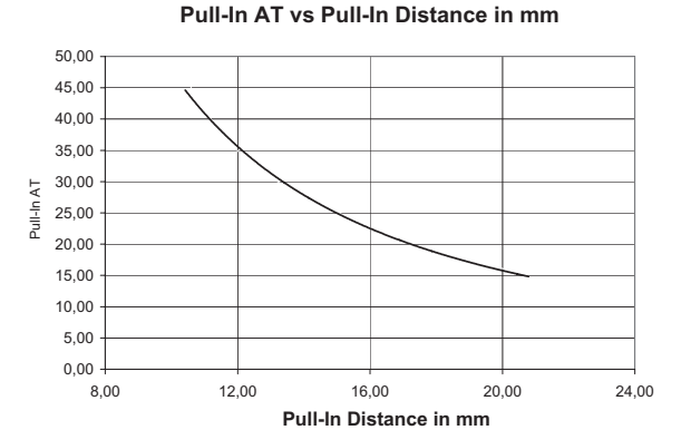
Fig. #8 The Pull-In AT is presented with its corresponding Pull-In distance from the magnet, and is measured in mm.
