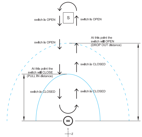
Fig. #29 Motion of the magnet is depicted in the y-z axis where the magnet is parallel to the Reed Switch, but moving perpendicular to its plane. The closure, holding, and opening points are shown.
