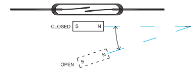
Fig. #23 A pivoting magnet is shown influencing the opening and closing points of a Reed Switch.
