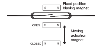
Fig. #34 A Reed Switch can be biased closed with a magnet. When a second magnet with an opposing magnetic field is brought close, the Reed Switch will open giving rise to a normally closed sensor.
