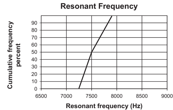
Fig. #17. A depiction of a group of 10 mm Reed Switches and its resonant frequency distribution.
