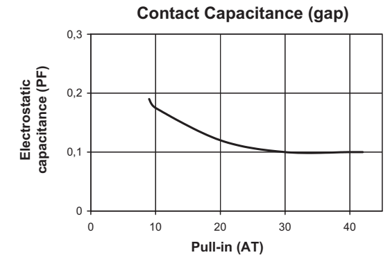
Fig. #18 As the Pull-in AT increases its gap increases, therefore reducing the capacitance across the Reed Switch.
